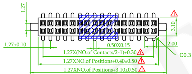
Inner Peg
