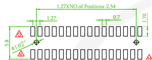
Inner Peg
