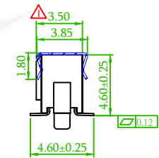
Outer Peg
