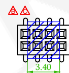
Special CAP for 2*2P 2*3P 2*4P W/O Bump
