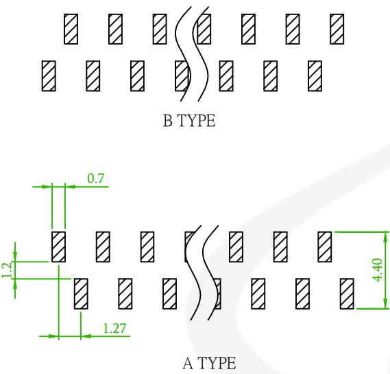
Recommended PCB Layout (PCB TOLERANCE ±0.05)
