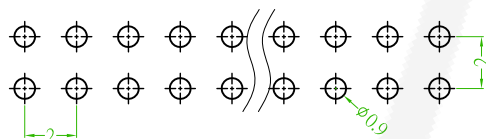
Recommended PCB Layout (PCB TOLERANCE ±0.1)
