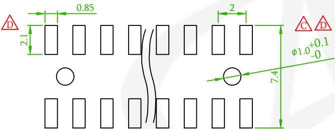
Recommended PCB Layout (PCB TOLERANCE ±0.05) △D
