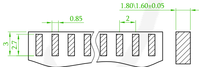
Recommended PCB Layout (PCB TOLERANCE ±0.1)
