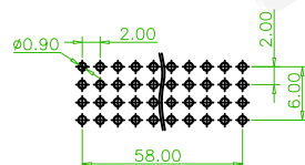
Recommended PCB Layout (PCB TOLERANCE ±0.1)
