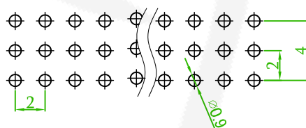
Recommended PCB Layout (PCB TOLERANCE ±0.1)
