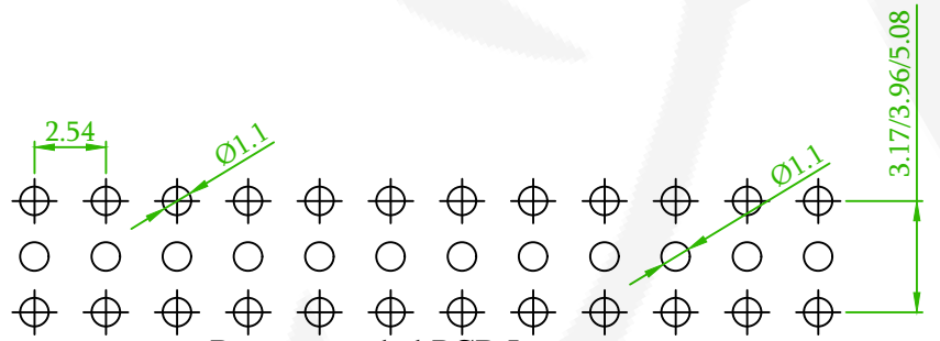
Recommended PCB Layout (PCB TOLERANCE ±0.1)
