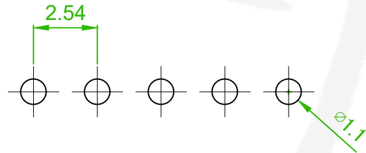
Recommended PCB Layout (PCB TOLERANCE ±0.1)
