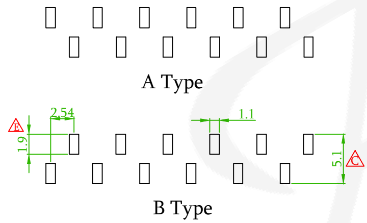
Recommended PCB Layout (PCB TOLERANCE ±0.05) \triangle A
