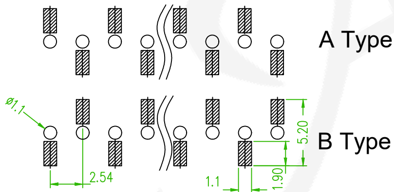
Recommended PCB Layout (PCB TOLERANCE ±0.1)
