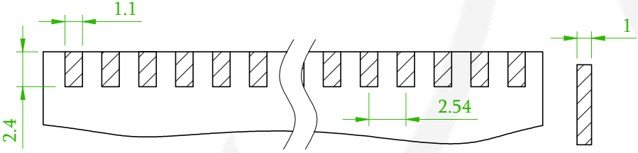
Recommended PCB Layout (PCB TOLERANCE ±0.1)
