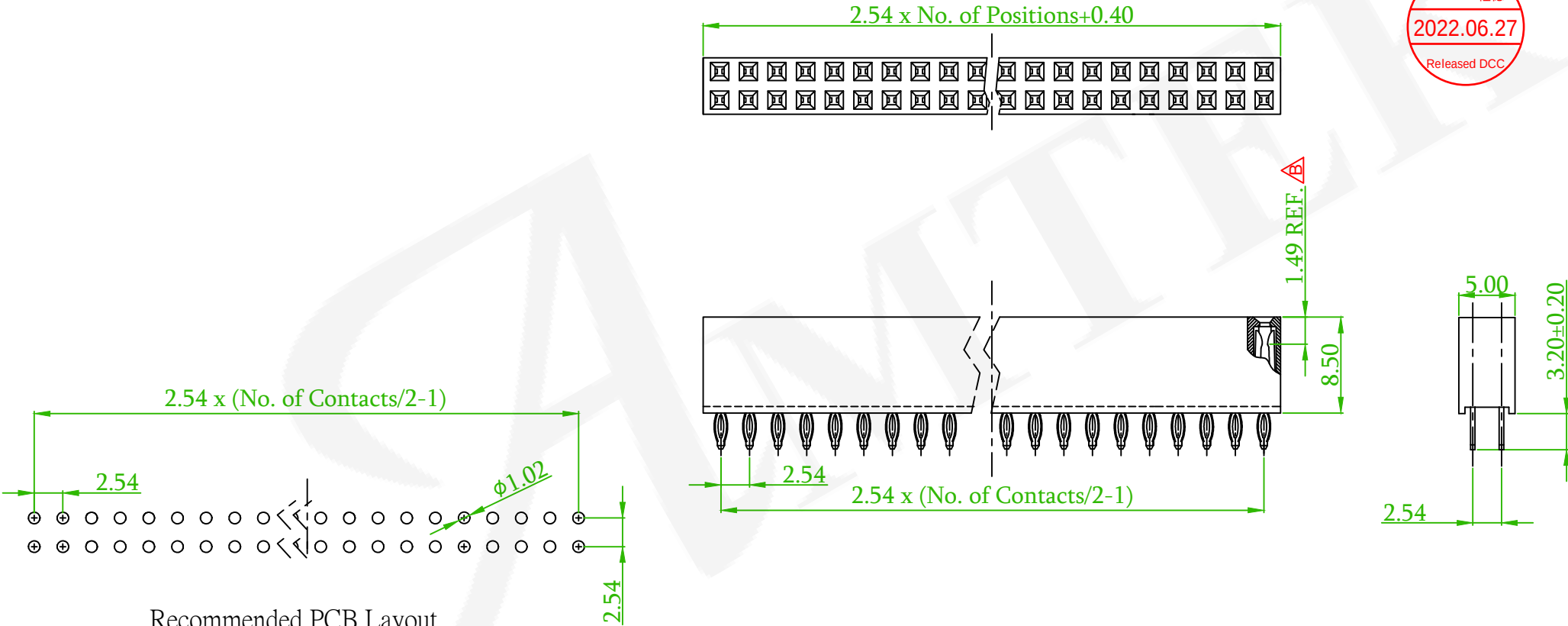
Recommended PCB Layout (PCB TOLERANCE \pm 0.1 )
