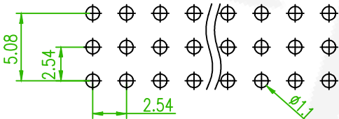
Recommended PCB Layout (PCB TOLERANCE ±0.1)
