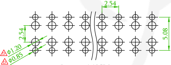
Recommended PCB Layout (PCB TOLERANCE ±0.05) ⚠
