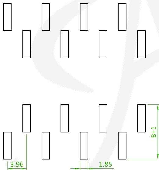
Recommended PCB Layout (PCB TOLERANCE ±0.1)
