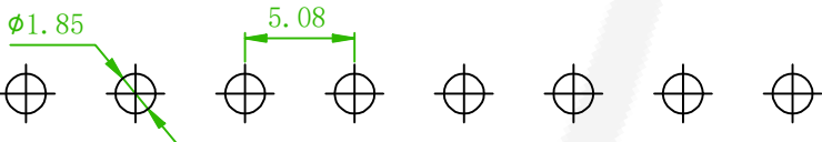
Recommended PCB Layout (PCB TOLERANCE ±0.05)
