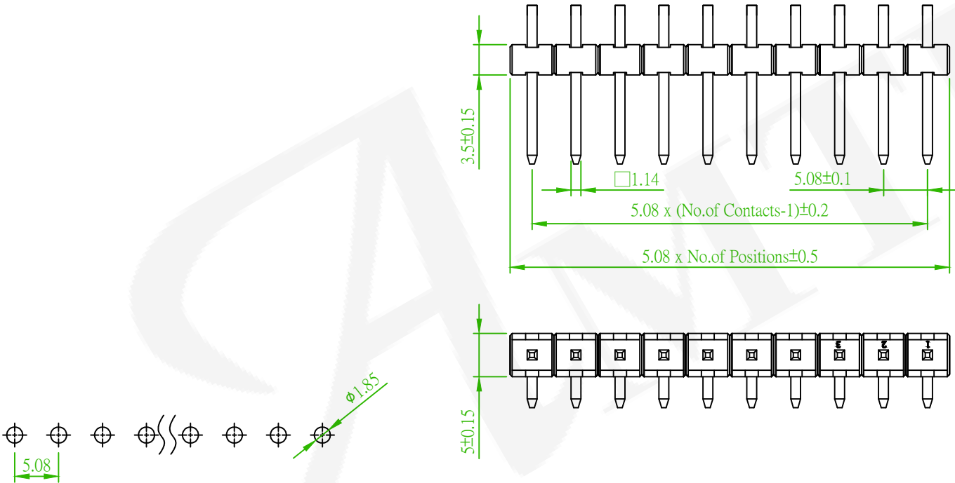
Recommended PCB Layout (PCB TOLERANCE ±0.05)
