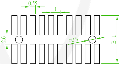
Recommended PCB Layout (PCB TOLERANCE ±0.1)
