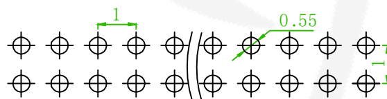
Recommended PCB Layout (PCB TOLERANCE ±0.1)
