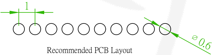
Recommended PCB Layout (PCB TOLERANCE ±0.05)
