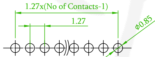
Recommended PCB Layout (PCB TOLERANCE ±0.1)
