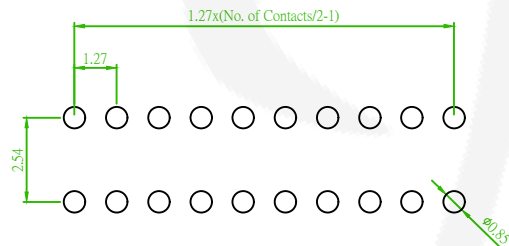
Recommended PCB Layout (PCB TOLERANCE ±0.1)
