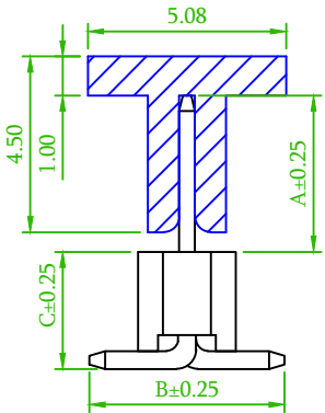
Old Part No. : PH4M25-1XX-U
