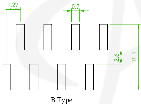
Recommended PCB Layout (PCB TOLERANCE ±0.1)
