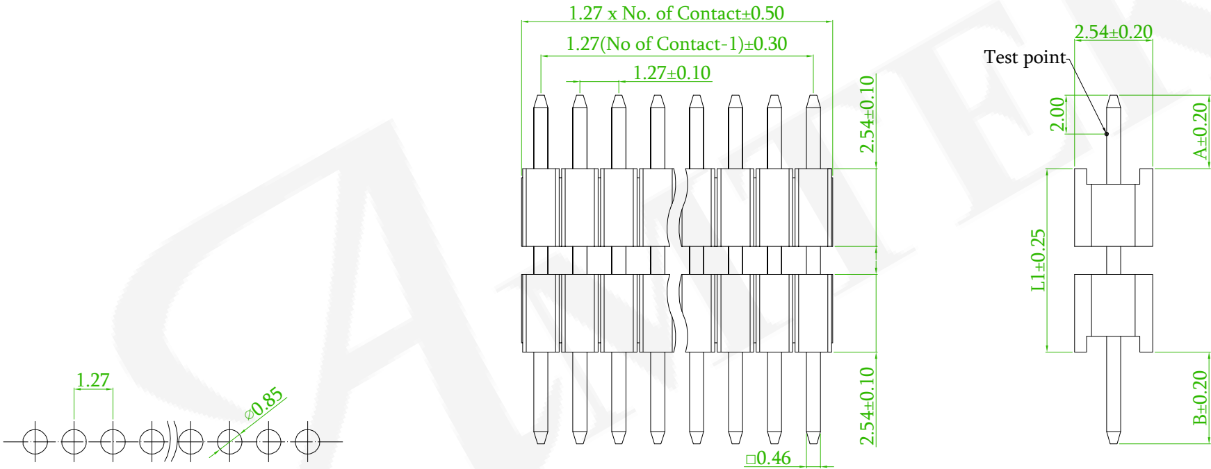
Recommended PCB Layout (PCB TOLERANCE ±0.05)
