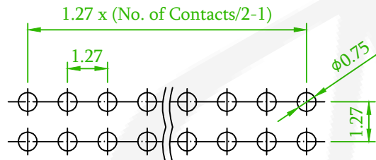
Recommended PCB Layout (PCB TOLERANCE \pm 0.1 )
