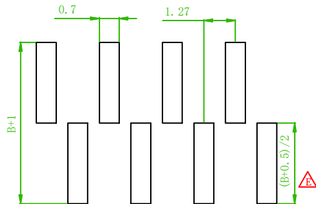
Recommended PCB Layout (PCB TOLERANCE ±0.1)
