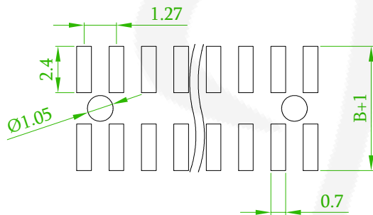
Recommended PCB Layout (PCB TOLERANCE \pm 0.05 )
