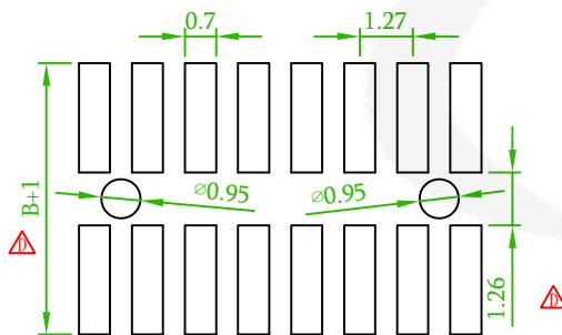
Recommended PCB Layout (PCB TOLERANCE \pm 0.1 )
