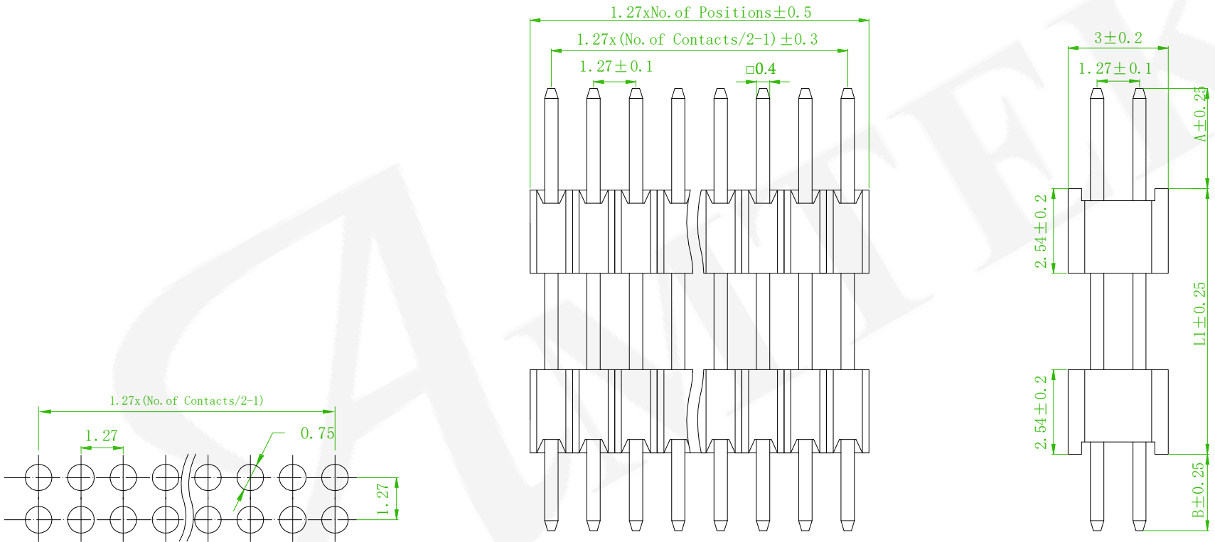
Recommended PCB Layout (PCB TOLERANCE ±0.05)
