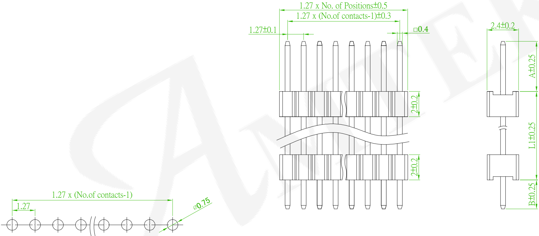
Recommended PCB Layout (PCB TOLERANCE ±0.05)
