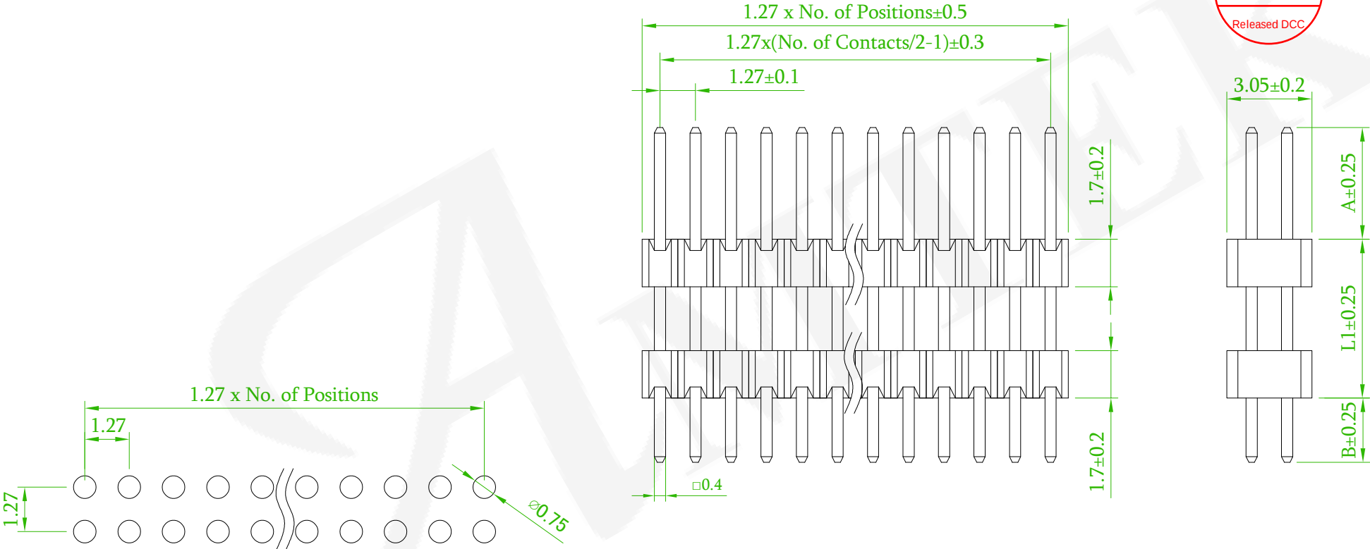
Recommended PCB Layout (PCB TOLERANCE ±0.05)
