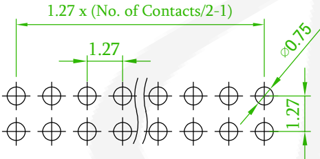
Recommended PCB Layout (PCB TOLERANCE ±0.1)
