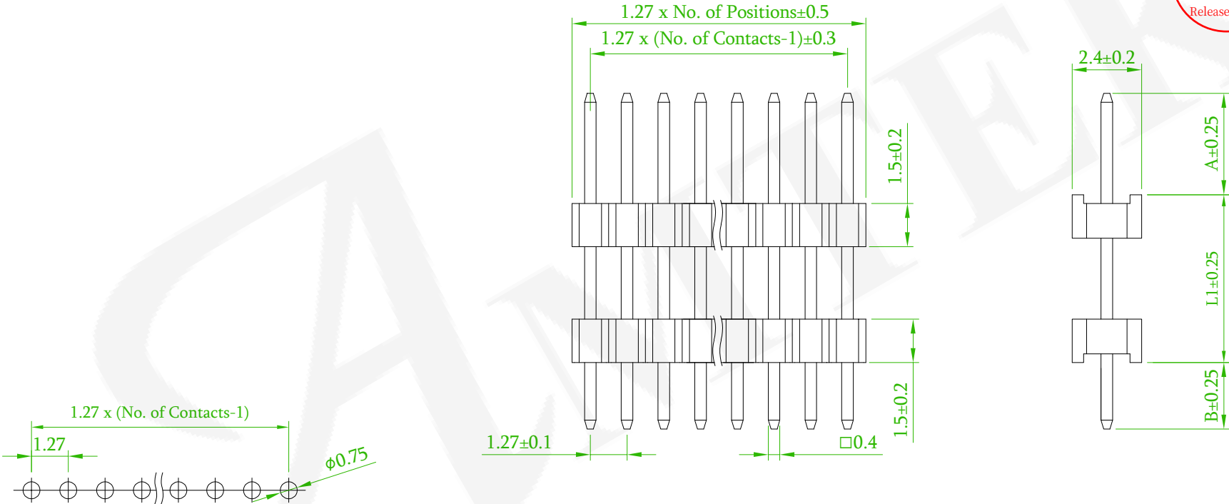
Recommended PCB Layout (PCB TOLERANCE ±0.05)
