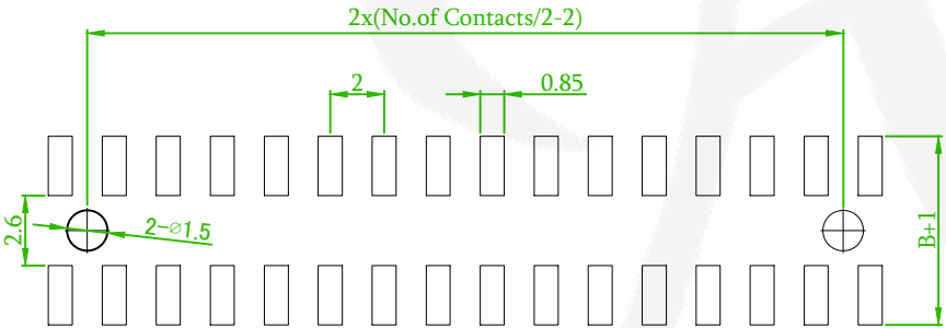
Recommended PCB Layout (PCB TOLERANCE ±0.1)
