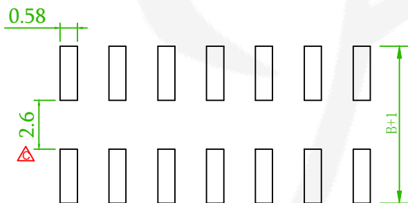
Recommended PCB Layout (PCB TOLERANCE \pm 0.1 )
