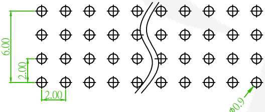
Recommended P.C.B Layout(Top Side) (PCB BOARD TOLERANCE±0.1)
