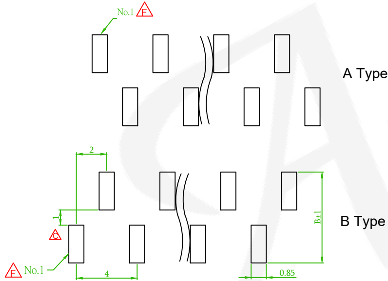
Recommended PCB Layout (PCB TOLERANCE ±0.1)
