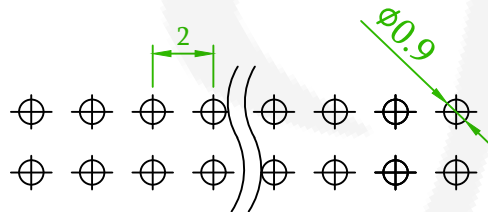
Recommended PCB Layout (PCB TOLERANCE \pm 0.1 )
