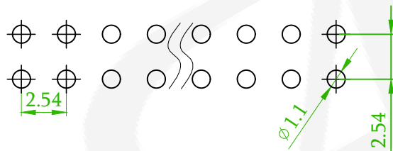
Recommended PCB Layout (PCB TOLERANCE \pm 0.1 )
