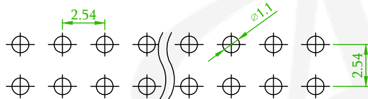
Recommended PCB Layout (PCB TOLERANCE ±0.1)
