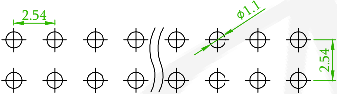
Recommended PCB Layout (PCB TOLERANCE ±0.1)
