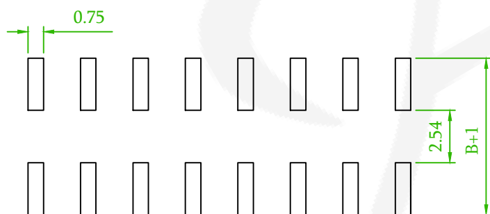
Recommended PCB Layout (PCB TOLERANCE \pm 0.05 )
