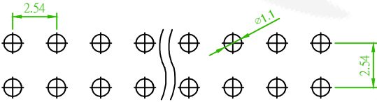
Recommended PCB Layout (PCB TOLERANCE ±0.1)
