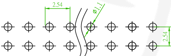
Recommended PCB Layout (PCB TOLERANCE ±0.1)
