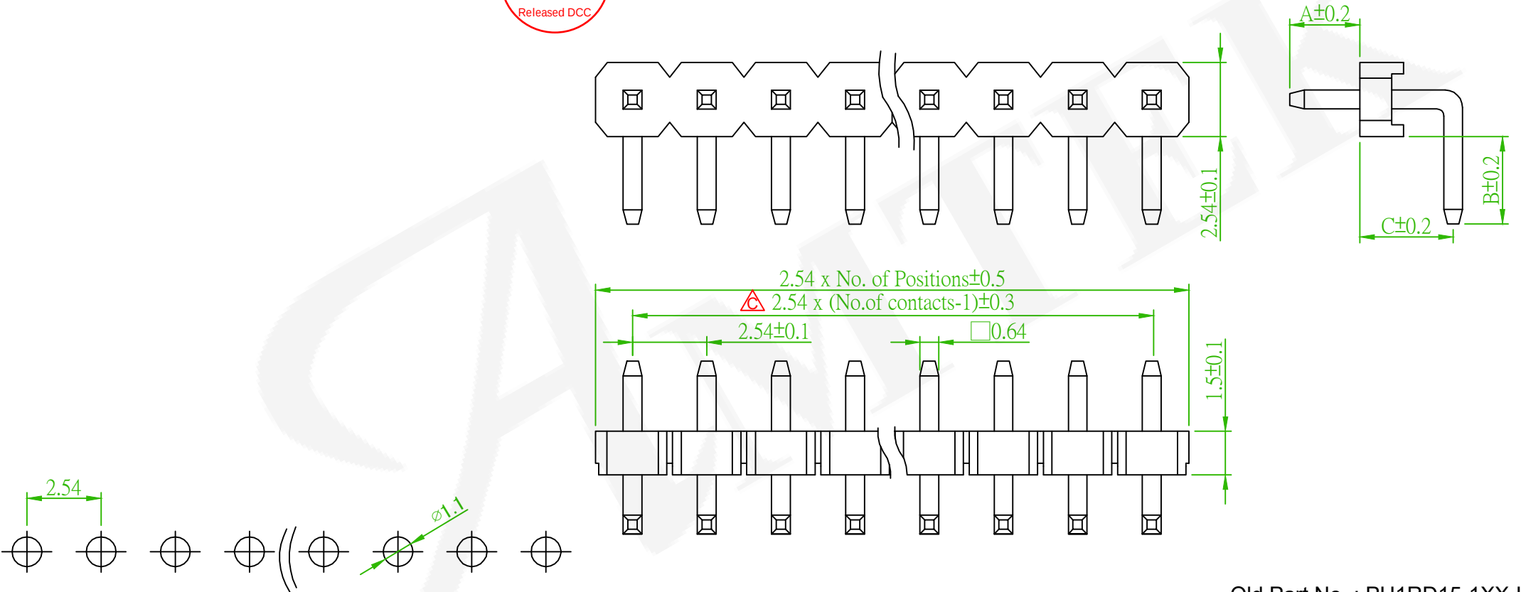
Recommended PCB Layout (PCB TOLERANCE ±0.05)
