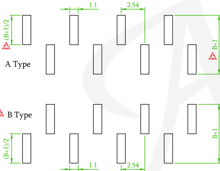
Recommended PCB Layout (PCB TOLERANCE ±0.1)
