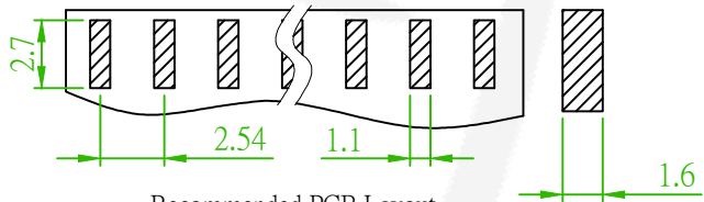
Recommended PCB Layout (PCB BOARD TOLERANCE±0.1)
