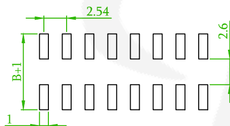
Recommended PCB Layout (PCB TOLERANCE ±0.1)
