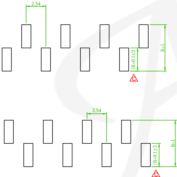
Recommended PCB Layout (PCB TOLERANCE ±0.1)
